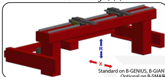
5 Axis Back Gauge (X,R,Z1,Z2, X Prime)
