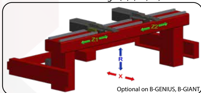
6 Axis Back Gauge (X1,X2,R1,R2,Z1,Z2)
